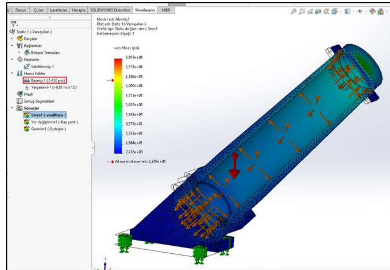
Barrel Static Analysis
